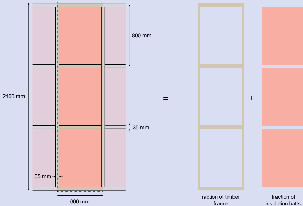
Figure E. 2 Insulation with framing acting as a thermal bridge
