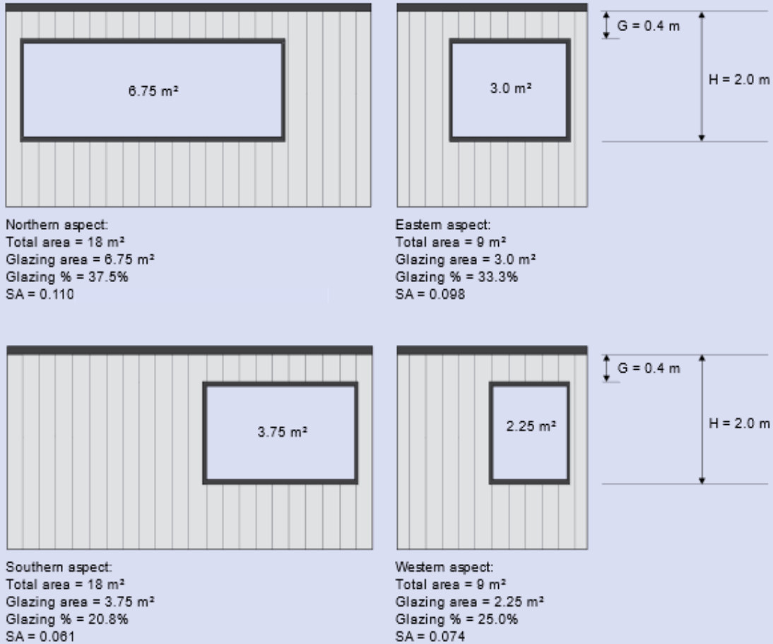
Figure E. 5 Window to wall ratio (multiple aspects)
